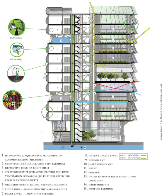
This "stackable" vertical farm was designed in Australia by ODESIGN.
